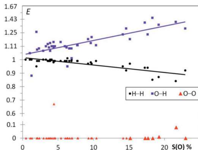
Figure 3 Contact enrichment ratios in crystals of ethers as a function of S_O .
