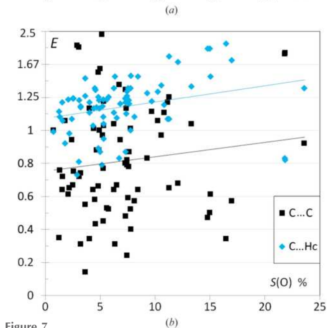
Figure 7 (a) Enrichment of O \cdots O , O \cdots Hc and O \cdots Ho contacts in phenols. Small symbols correspond to cases where the equiprobable contacts Rxy are smaller than 2%. (b) Enrichment ratios for the hydrophobic contacts types C \cdots Hc and C \cdots C .
